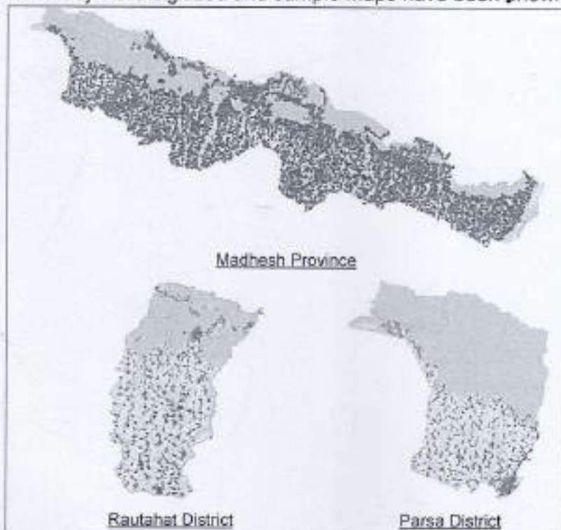
Figure 2-12: Digitized Houses
