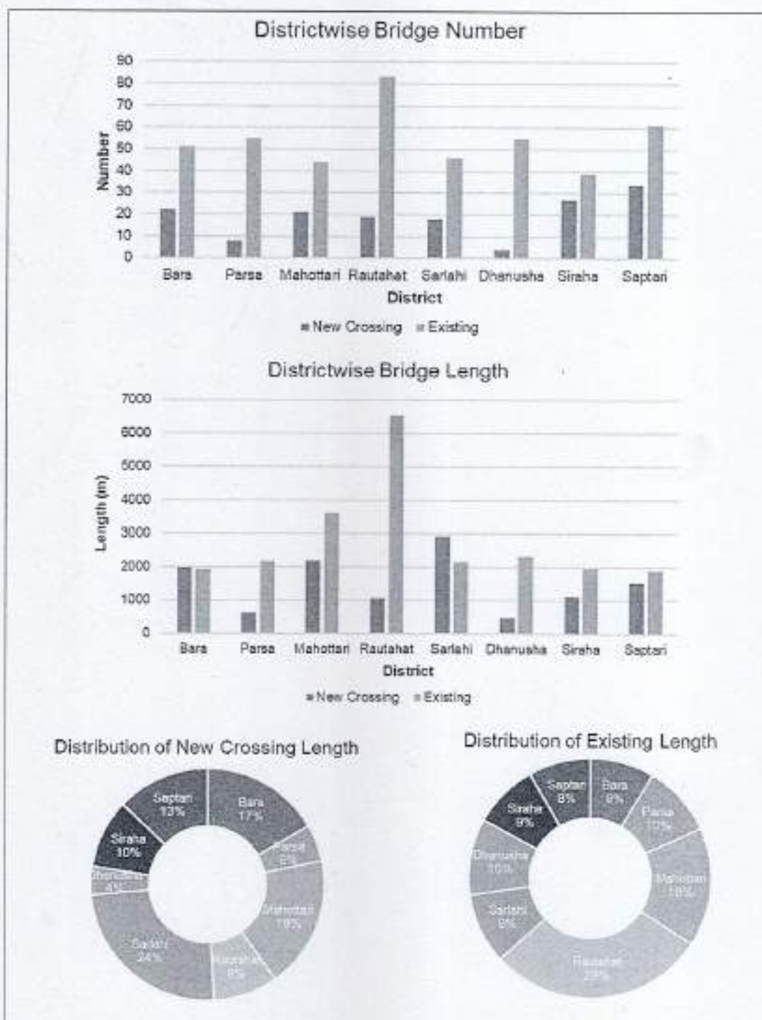
Figure 2-22: District wise Distribution of Bridges
