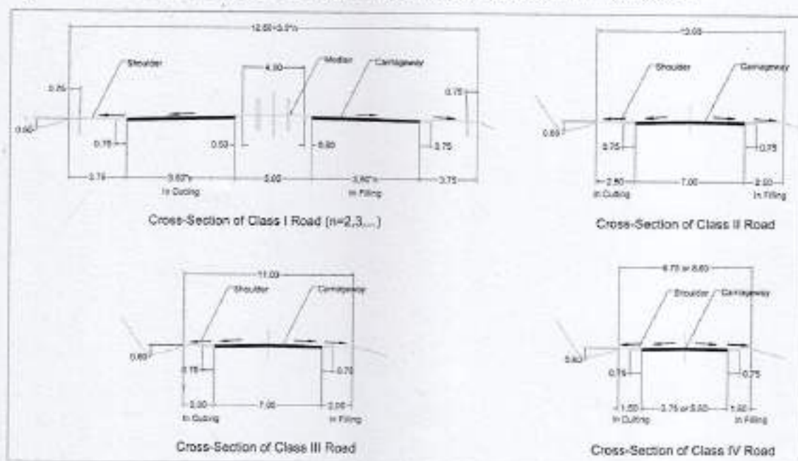
Figure 2-1: Typical Road Sections under Functional Classification
